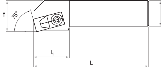
CSKNR/L.....12S
