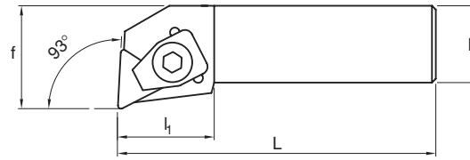
CTUNR/L.....16S
