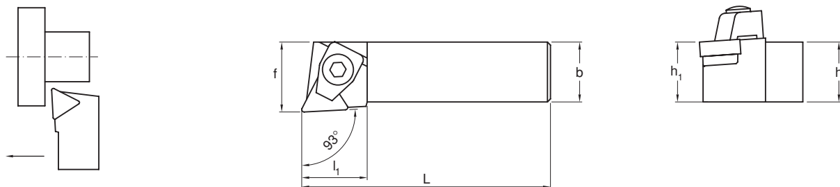
CTJNR/L.....16S
