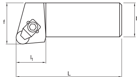
CRSNR/L.....12S
