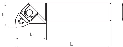
MWLN 95°
